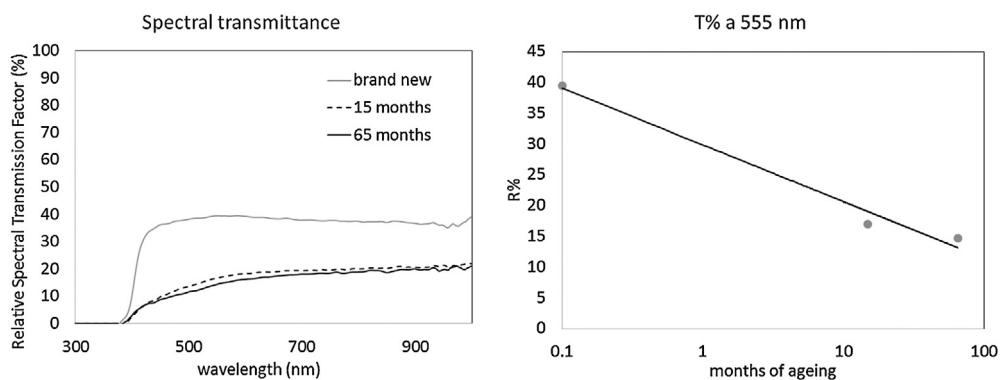
Fig. 7. Relative spectral transmittance of the textile samples, obtained by using 1% transmittance that diffuses the reference standard (left). Fit of the spectral reflection factor measured at 555 nm wavelength. Data shows a logarithmic trend (right).
