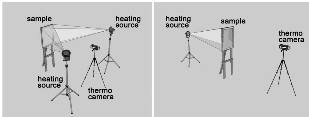
Fig. 1. Scheme of the measurement experimental set-up. In the reflection mode, samples were placed in front of both the camera and the heating at 45° to the normal of the sample surface (left). In transmission mode, samples were placed with a single back-heating source (right).
